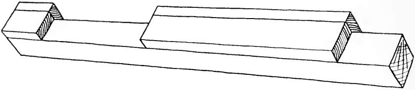
FIG. 391. BUILT-UP LEG.
